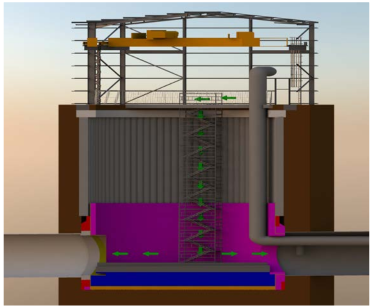
Shaft structure
